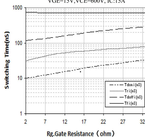
Switching Time vs. Rg(175°C)
